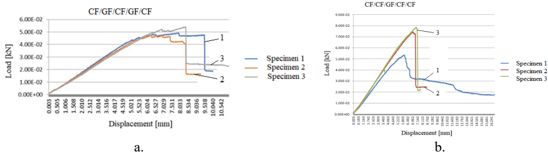
Fig. 6. Diagram Load-Displacement bending tests for 3 first specimens made by laminate: I: [CF/GF/CF/GF/CF] and II: [CF/CF/GF/CF/CF]
