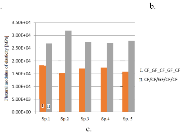
Figure 7. Numerical values determined experimentally in the bending test for hybrid laminates I and II: a. maximum resistance; b. maximum stress; c. flexural modulus of elasticity
