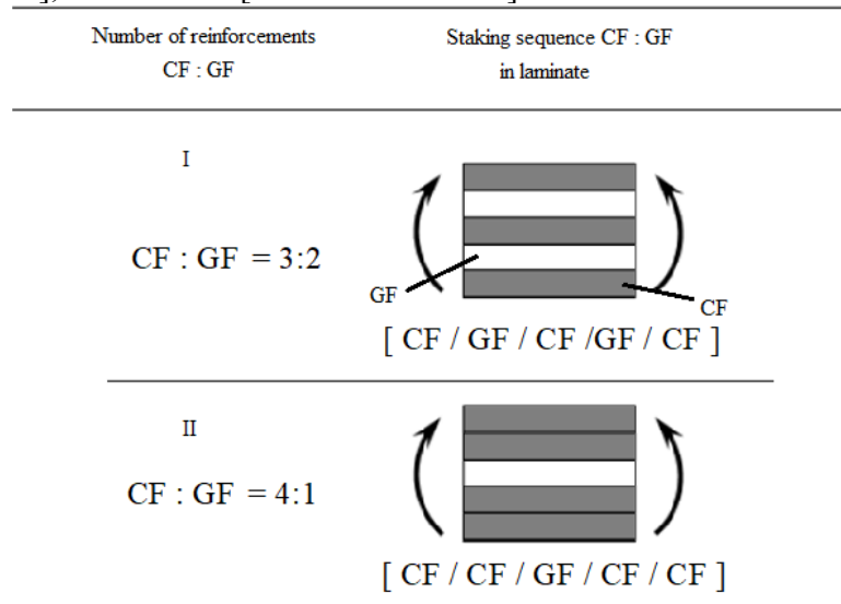
Figure 2. Laminate I (CF: GF 3: 2) and II (CF: GF = 4: 1) stacking sequences The two plates were made (Figure 3) By the Liquid Resin Infusion (LRI) technique [20].
